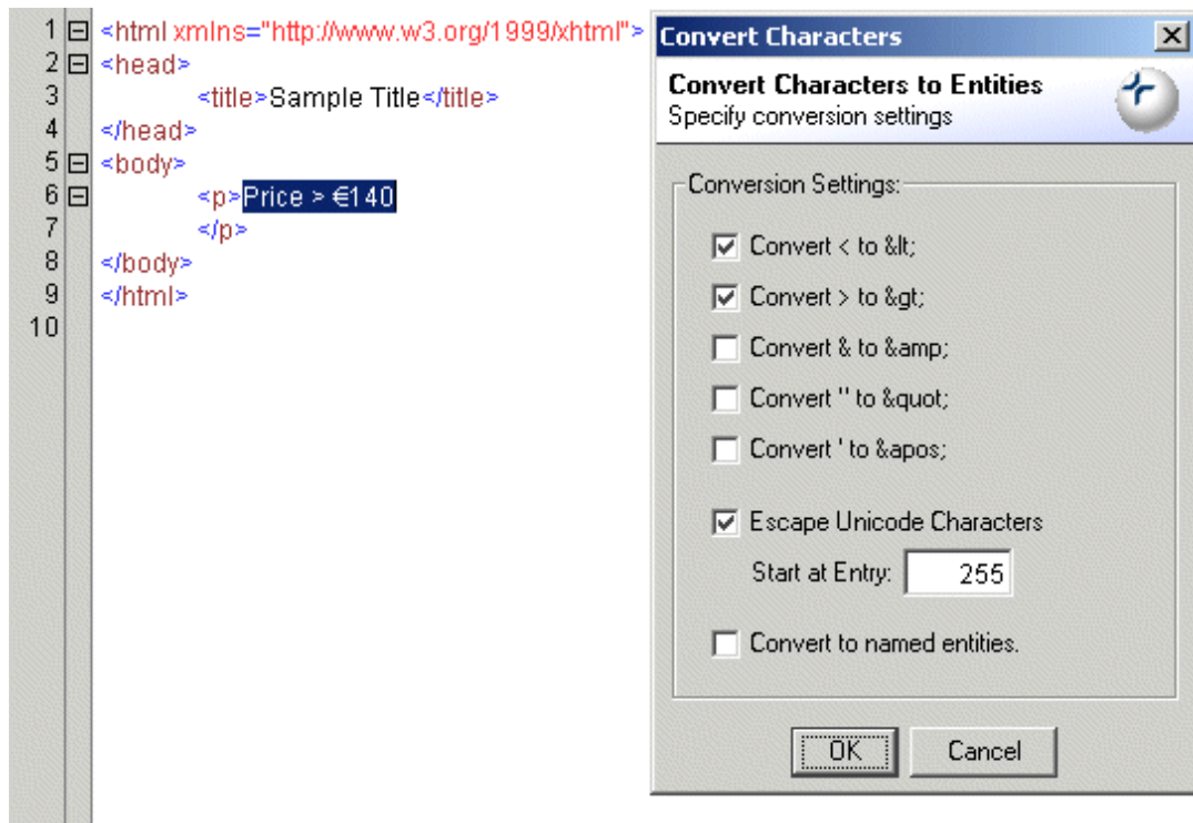
Figure 21. Convert Characters to Entities
