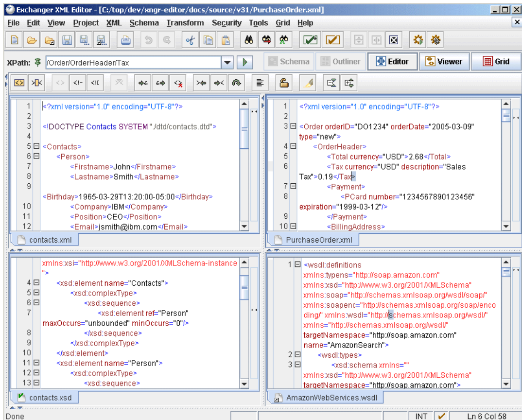
Figure 1. Splitting Windows Vertically and Horizontally
