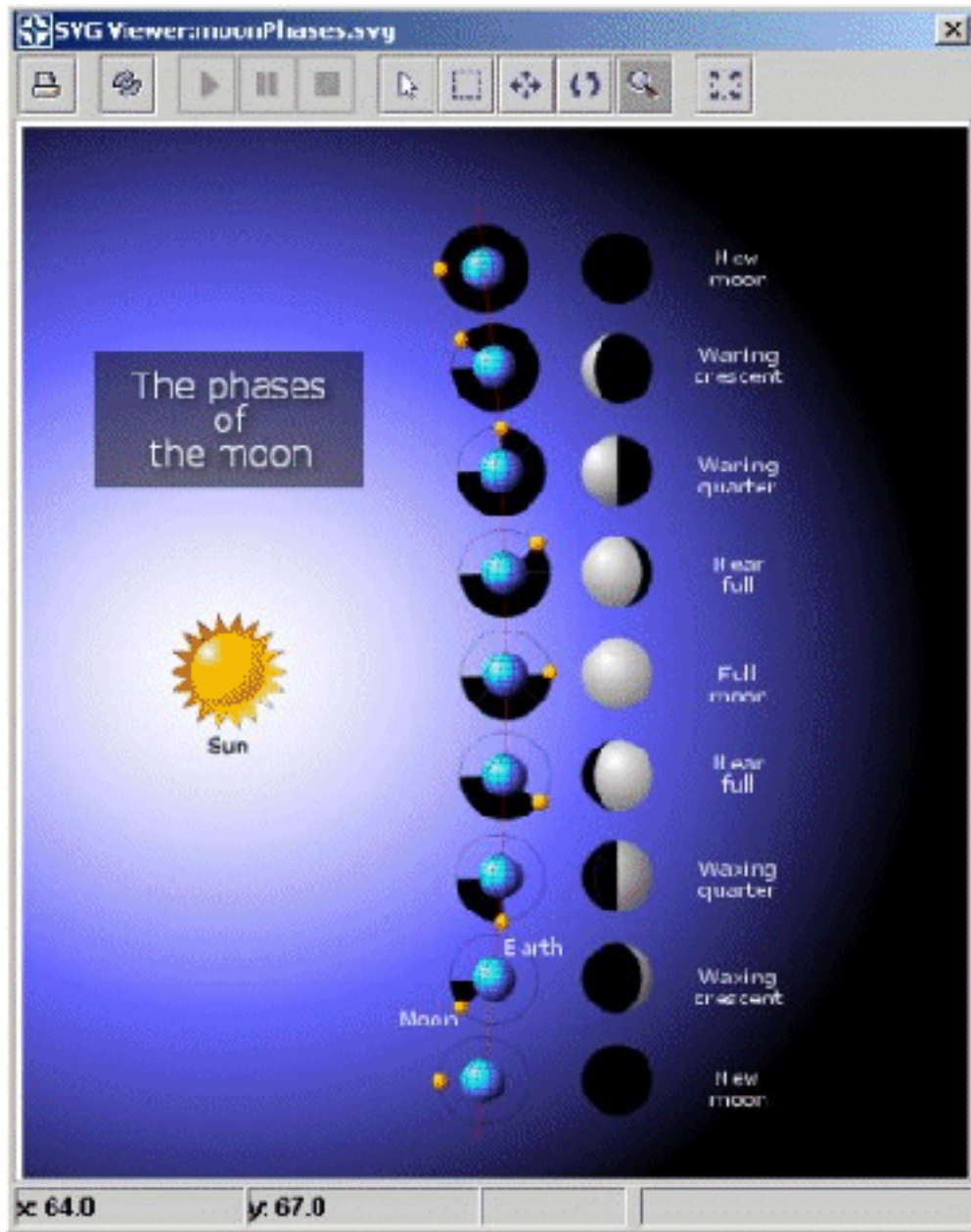
Figure 1. Viewing SVG
