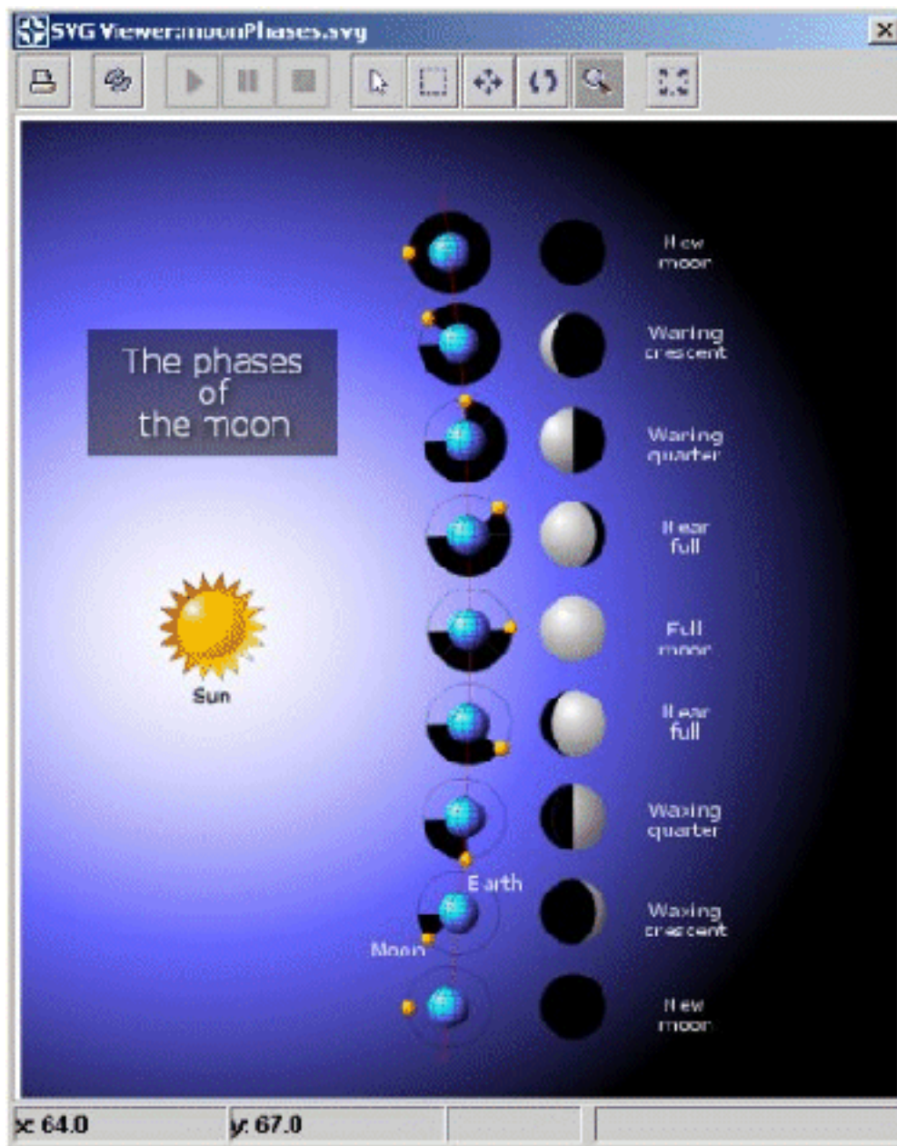
Figure 1. Viewing SVG
